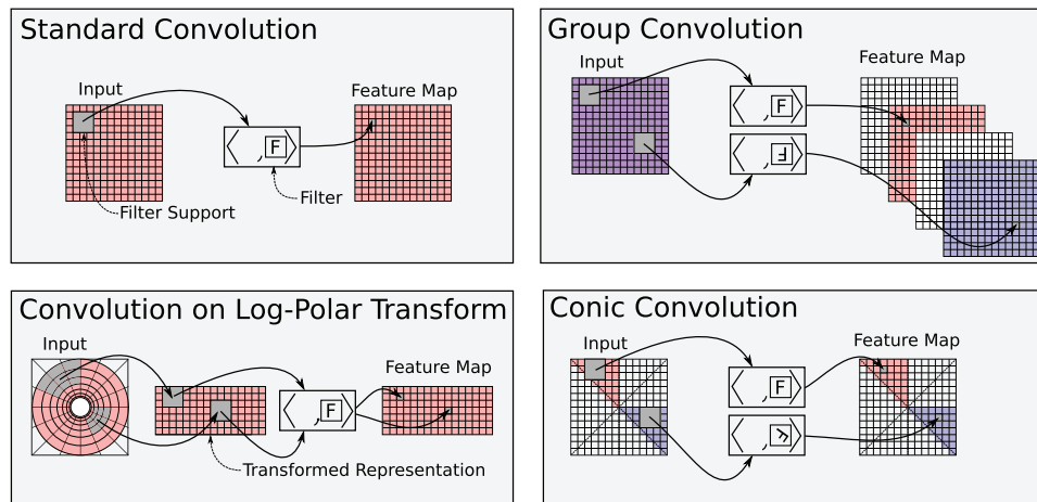
Fig. 1. Comparison of convolution schemes. The domain of filter ‘F’ in the input and its corresponding outputs in the feature map are colored red. That of the rotation of ‘F’ by 225 degrees is colored blue. The local support on the domain for the convolution at a few points for each scheme is shown in gray. Conic convolution, with rotations of 45 degrees in this example, encodes rotation equivariance without introducing distortion to the support of the filter in the original domain (unlike the log-polar transform) and without requiring additional storage for feature maps (unlike group convolution). The example shown for group convolution is the first layer of a G-CNN, mapping from \mathbb{Z}^2 to the roto-translation group
