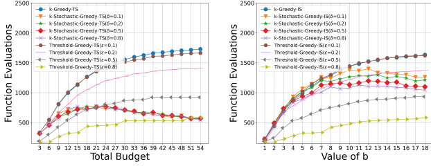
(c) Comparison of function queries for TS constraints. (d) Comparison of function queries for IS constraints.
