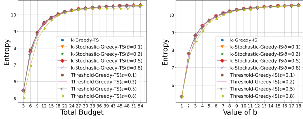
(a) Entropy comparison for TS constraints. (b) Entropy comparison for IS constraints.
