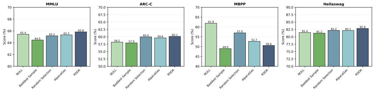
Figure 5: Results on the Databricks-Dolly dataset validating the reusability of low-quality data. “NULL” denotes the original Meta-Llama-3-8B model without fine-tuning.
