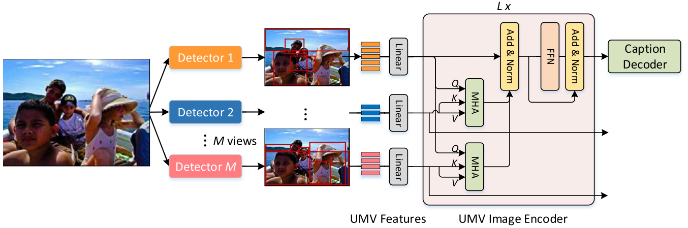
Fig. 3. The flowchart of the unaligned multi-view (UMV) image encoder model. Given an image, unaligned multi-view features are extracted from different object detectors in parallel. The unaligned multi-view features are fed into the UMV model to output the attended features with adaptive alignment learning.
