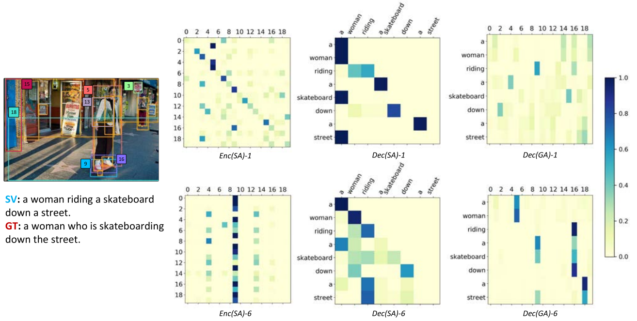
Fig. 5. Visualizations of the 1st and 6th attention maps ( \text{softmax}(QK/\sqrt{d}) ) of the MT_{sv} model with R-101 backbone. Enc(SA) denotes the self-attention in the image encoder; Dec(SA) and Dec(GA) denote the self-attention and guided-attention in the caption decoder, respectively. GT denotes the one of the five ground-truth captions provided by MSCOCO. The index within [0-19] shown on the axes of the attention maps corresponds to each object in the image (20 objects in total). For better visualization effect, we highlight some objects in the image that receive large attention values.
