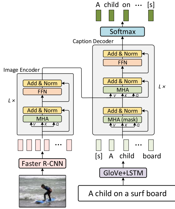
Fig. 1. Multimodal Transformer (MT) model for image captioning. It consists of an image encoder to learn self-attended visual features, and a caption decoder to generate the caption from the attended visual features. [s] is a delimiter that indicates the start or the end of the caption.
