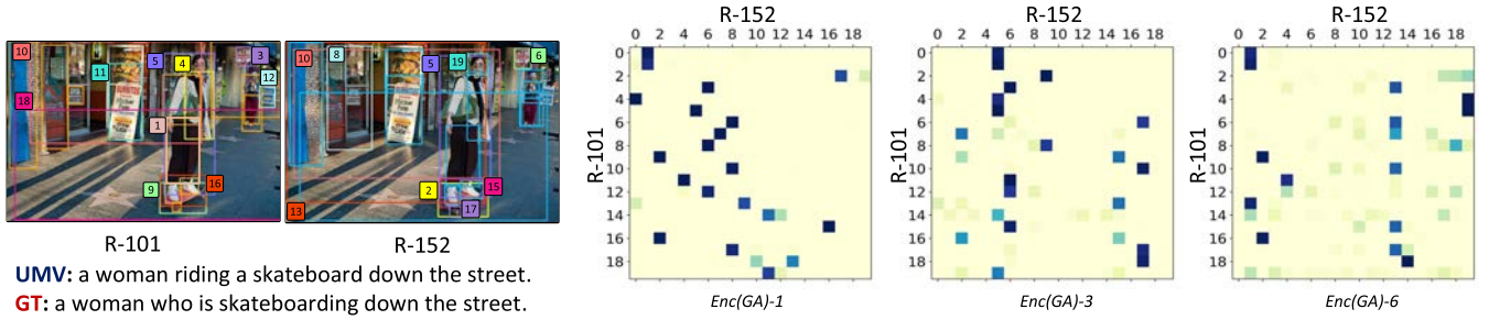
Fig. 6. Visualizations of the 1st, 3rd and 6th attention maps of the MT_{UMV} model with R-101 and R-152 backbones. Enc(GA) denotes the guided-attention in the UMV image encoder (i.e., the cross-view attention within the MHA module in Fig. 3).
