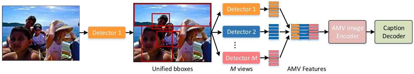
Fig. 2. The flowchart of the aligned multi-view (AMV) image encoder model. Given an image, different object detectors are regarded as the multiple views. To obtain the aligned multi-view features, we choose one of the M detectors to predict the unified bounding boxes for objects, and then use these bboxes to extract aligned multi-view features. The aligned multi-view features are fed into the AMV image encoder (which is exactly the same as the one for single-view features introduced in section III-B).
