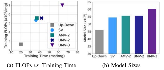
Fig. 4. Ablations of the computational costs of the MT models with different visual features. SV, AMV-2, UMV-2, UMV-3 denotes the the single-view features (R-101), aligned multi-view features (R-101 and R-152), unaligned multi-view features (R-101 and R-152), unaligned multi-view features (R-101, R-152 and X-101), respectively. For each model, we report the average training FLOPs vs. training time per one image in (a) and its corresponding model size in (b). Up-Down [6] is a strong reference image captioning model. (a) FLOPs vs. Training Time. (b) Model Sizes.
