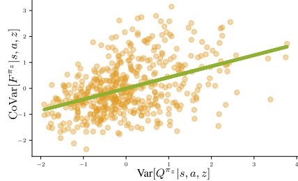
Figure 5: Regression scatter plot of the trace of \text{CoVar}[F^{\pi_z} | s, a, z] and \text{Var}[Q^{\pi_z} | s, a, z] for a FB checkpoint in Maze experiment.
