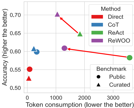
Figure 3: Overall benchmark performance of different methods.
