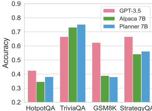
Figure 6: Performance alternating LLMs in ReWOO. Planner 7B is tuned on HotpotQA and TriviaQA
