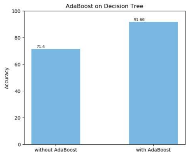
Fig-6: AdaBoost on Decision Trees
