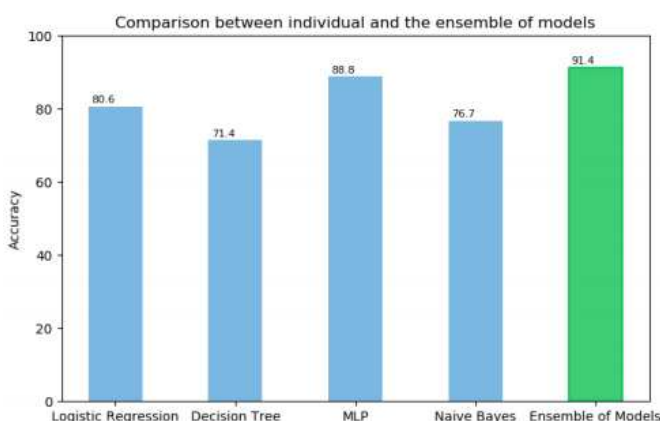
Fig-7: Final Comparison of accuracies
