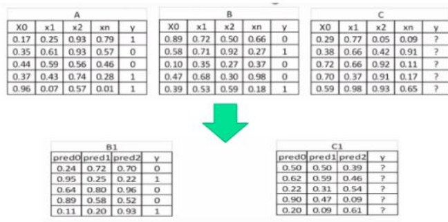
Fig-5: Displays the process of ensembling
