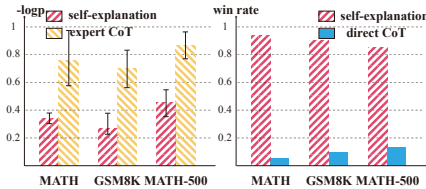
Figure 2: Left: Negative log-likelihood of the self-explanation \tilde{c} and expert CoT. Right: Winrate labelled by GPT-4o in terms the number of correct steps of the self-explanation \tilde{c} and self-generated CoT c . Both on the test split of each dataset using Qwen2.5 3B-Instruct.
