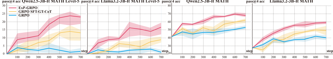
Figure 3: Accuracy on the level-5 questions from MATH test set (left 1, 2) and on the whole test set (right 3, 4) for Qwen2.5-3B-Instruct and LLaMA-3.2-3B-Instruct across global training steps. ExP-GRPO consistently outperforms both GRPO and GRPO SFT-GT-CoT , the latter uses supervised fine-tuning on expert CoT c_E . The results show that ExP-GRPO provides more effective and generalizable learning signals, leading to improved sample efficiency and higher overall performance.
