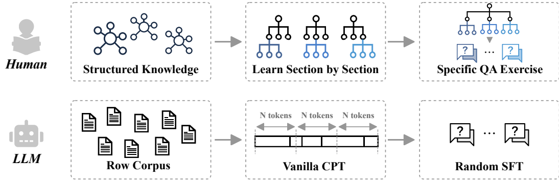
Figure 1: Discrepancy between human education and vanilla LLM adaptation. Human students learn structured knowledge through textbooks section by section, with particular exercises on related knowledge points. Traditional LLM adaptation continually pre-trains on data chunks from randomly concatenated text segments, with aimless supervised fine-tuning for conversation alignment. The inherent knowledge structure is ignored.
