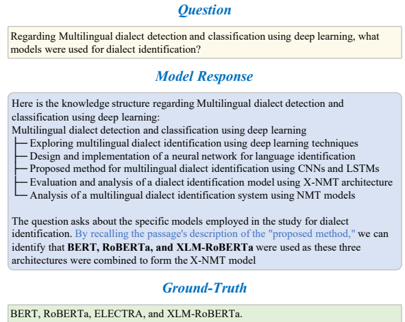
Figure 5: An example for structure-aware responses.
