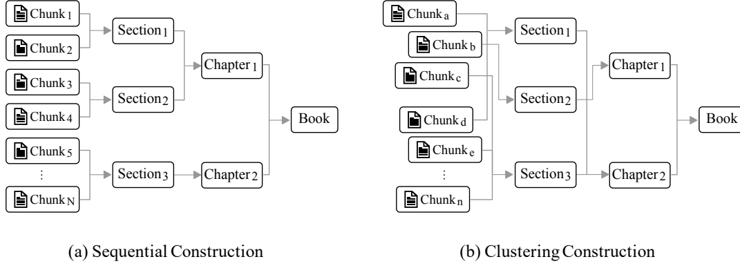
Figure A1: Knowledge structure extraction from (a) sequential chunks ( e.g. , from textbooks) by our specialized 7B model and (b) separated trunks ( e.g. , from websites) by clustering-based methods (Sarathi et al., 2024). Here the terms of “Section”, “Chapter”, and “book” are just examples to help illustrate the knowledge structure.
