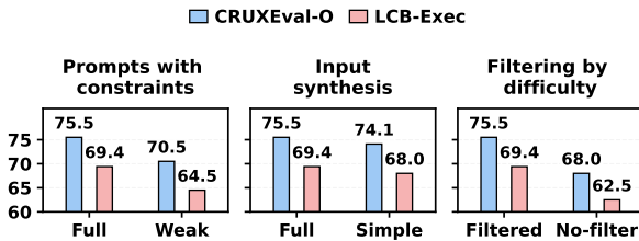
Figure 4: Ablation study on our synthesis pipeline on CRUXEval-O and LiveCodeBench-Exec. We report pass@1 on models finetuned with different data synthesis variants.
