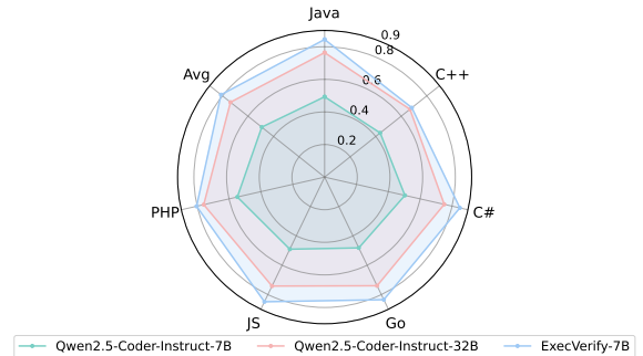
CruxEval-X I/O Prediction (Multi-lingual)
