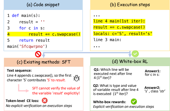
Figure 1: Comparison between SFT and white-box RL. (a) Code snippet. (b) Execution steps extracted from the interpreter, with the relevant parts highlighted in yellow. (c) SFT optimizes the cross-entropy loss over the entire sequence, without explicitly verifying execution details like variable values or control flow. (d) In contrast, white-box RL leverages interpreter-provided execution steps to assign verifiable and step-level rewards.
