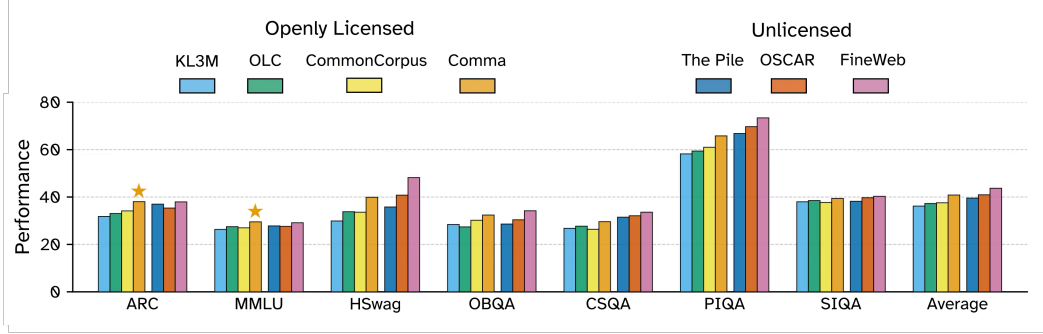
Figure 2: The Common Pile consistently outperforms other openly licensed corpora as a pre-training dataset. Following the setup from Penedo et al. [133], we train and evaluate 1.7B parameter models on 28B tokens of data from each dataset. Stars denote benchmarks on which the model trained using the Common Pile outperforms all other models.
