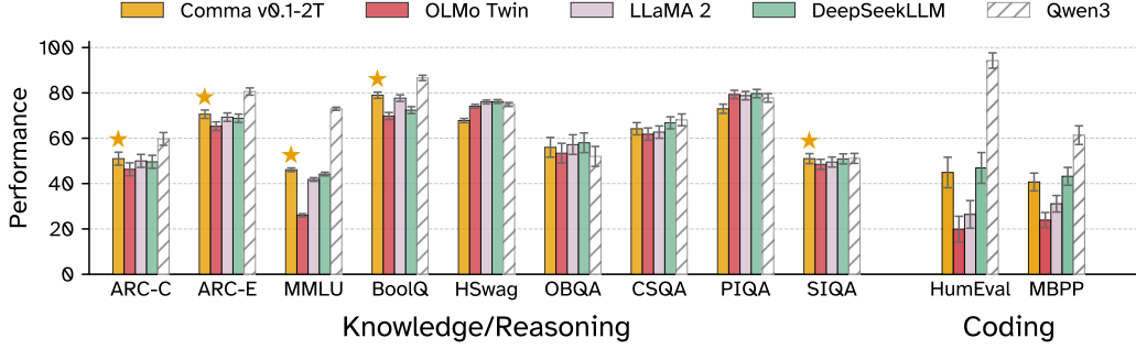
Figure 4: Comma v0.1-2T is also competitive with budget-matched models (7 billion parameters, 2 trillion tokens) trained on unlicensed data. We additionally include Qwen3 8B as a higher budget upper bound. Stars denote benchmarks where Comma v0.1-2T achieves the highest score among compute-matched models. Full numerical results are provided in Table 11 (appendix).
