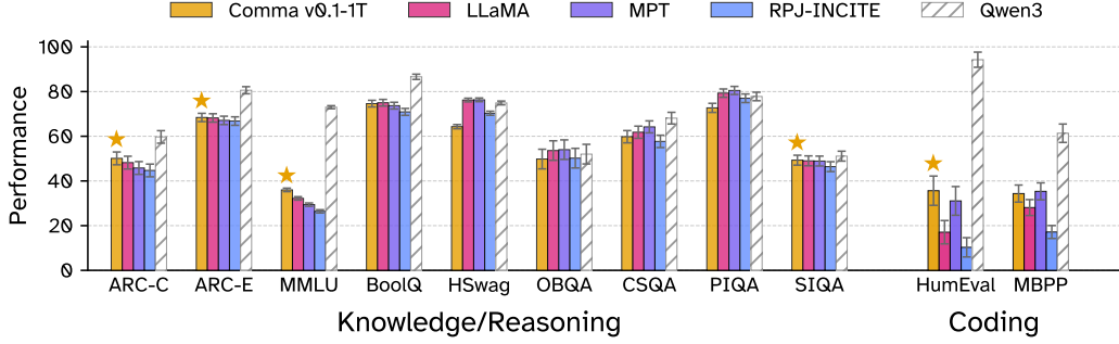
Figure 3: Comma v0.1-1T performs comparably to models trained with similar resources (7 billion parameters, 1 trillion tokens) on several standard benchmarks. To contextualize these results, we include Qwen3 8B (trained on 36 trillion tokens) as a “current best-practices” upper bound. Stars denote benchmarks on which Comma v0.1-1T achieves the highest score among compute-matched models (i.e., all models other than Qwen3). Error bars represent 95% confidence intervals. Full numerical results are provided in Table 10 (appendix).
