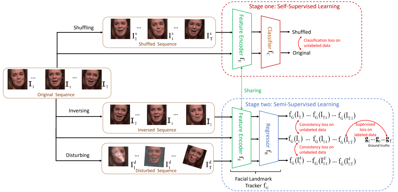
Figure 1: The proposed two-stage learning framework. The first stage is self-supervised learning stage, as shown in the upper part of the figure. The second stage is semi-supervised learning stage, as shown in the lower part of the figure.
