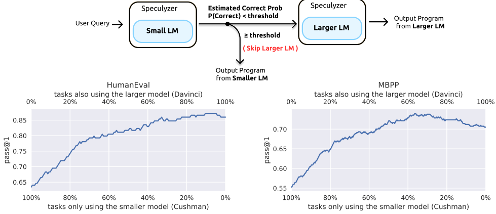
Figure 5: Mixing small cheap models and large powerful models by delegating to the large model only those problems that our approach thinks that the small model cannot solve. There are some MBPP problems where small model beats the big one. Our method multiplexes correctly for those.
