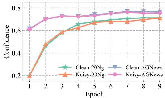
Figure 1: The average confidence of clean and noisy samples during fine-tuning BERT on datasets 20Ng and AGNews with 20% noisy labels.
