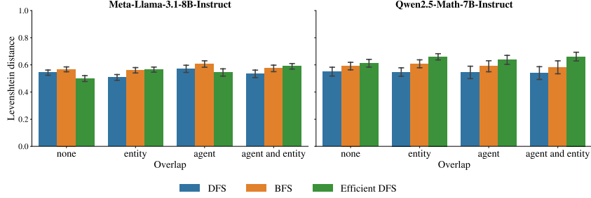
Figure 8: Average Levenshtein distance between Llama-3.1-8B-Instruct’s search order and depth-first search (DFS), breadth-first search (BFS), and an efficient DFS which only visits relevant theorems. The plot is based on problems for which the model gave the correct answer. The Levenshtein distances are normalized by the length of the longest string to take values in [0, 1] ; lower values mean shorter distances.
