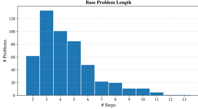
Figure 4: Histogram of the number of inference rule applications required in the most efficient proof for the GSM problems in our dataset.
