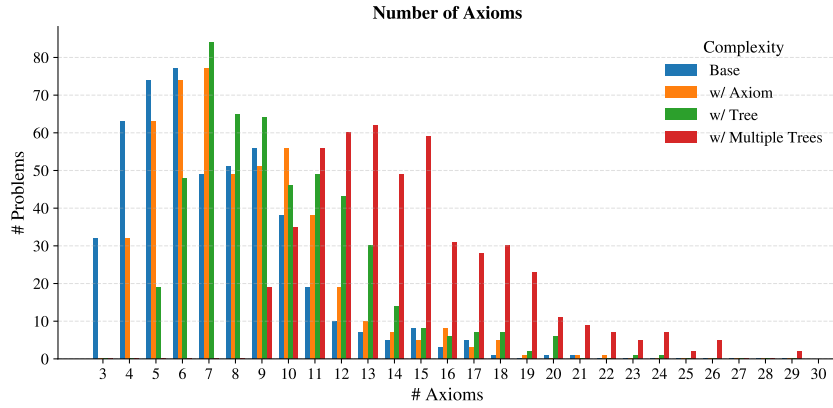
Figure 5: Histogram of the total number of axioms, including irrelevant ones, per type of complexity of the GSM problems in our dataset.
