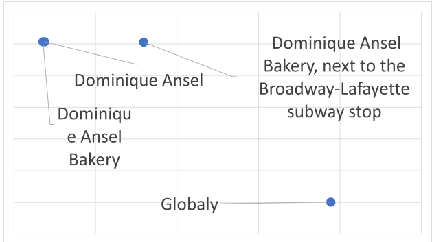
Figure 2: An example of the 2D UMAP (McInnes et al., 2018) projection of the embeddings used in Ecc for 20 responses. The question and answer are “Q: What is the bakery’s name? A:the Dominique Ansel Bakery”. Similar answers tend to live closely together, justifying the use of distance-based uncertainty and confidence measures ( U_{\text{Ecc}} and C_{\text{Ecc}} ).
