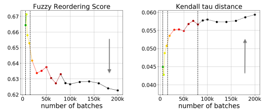
Figure 13: (a) fuzzy reordering score (for references: 0.5), (b) Kendall tau distance (for references: 0.08); WMT En-De. The arrows point in the direction of less monotonic alignments (more complicated reorderings).
