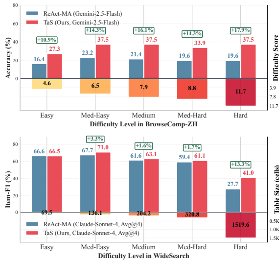
Figure 2: Robustness Analysis on BrowseComp-ZH (Top) and WideSearch (Bottom).
