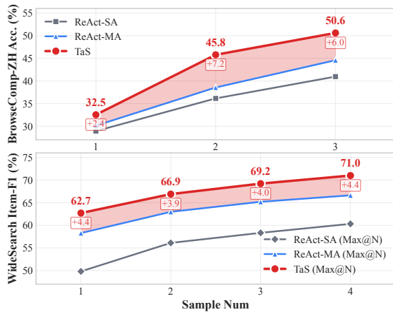
Figure 4: Test-time Scaling Analysis on BrowseComp-ZH (Top, Gemini-2.5-Flash) and WideSearch (Bottom, Claude-Sonnet-4).
