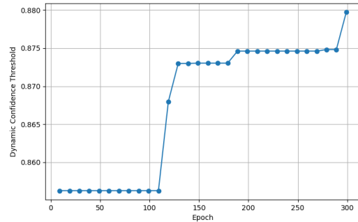
Figure 7: Dynamic changes in confidence threshold during training for VLK-RL (Qwen14b).
