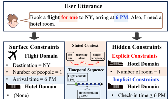
Figure 1: Example of explicit (traveling alone implies single-occupancy accommodation) and implicit (hotel check-in must follow flight arrival) constraints in a cross-domain scenario.
