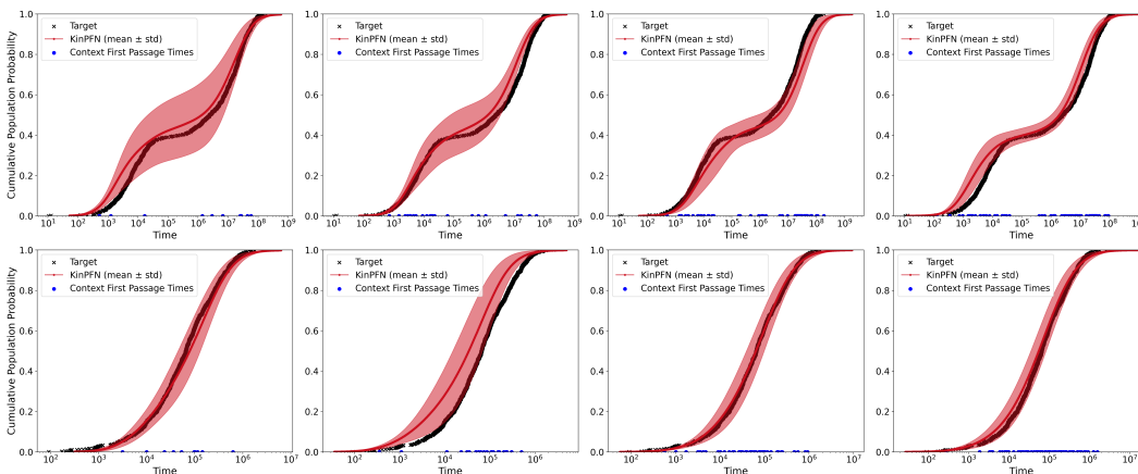
Figure 15: KinPFN first passage time CDF approximations with context times N \in \{10, 25, 50, 75\} (left to right) for Saccharomyces cerevisiae tRNA phe (top) and 5S rRNA (bottom).
