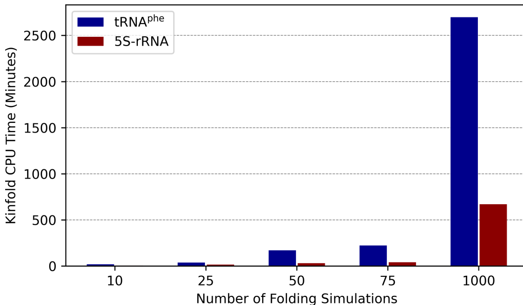
Figure 16: Kinfold CPU time (in minutes) vs. number of folding simulations for Saccharomyces cerevisiae tRNA phe and 5S rRNA.
