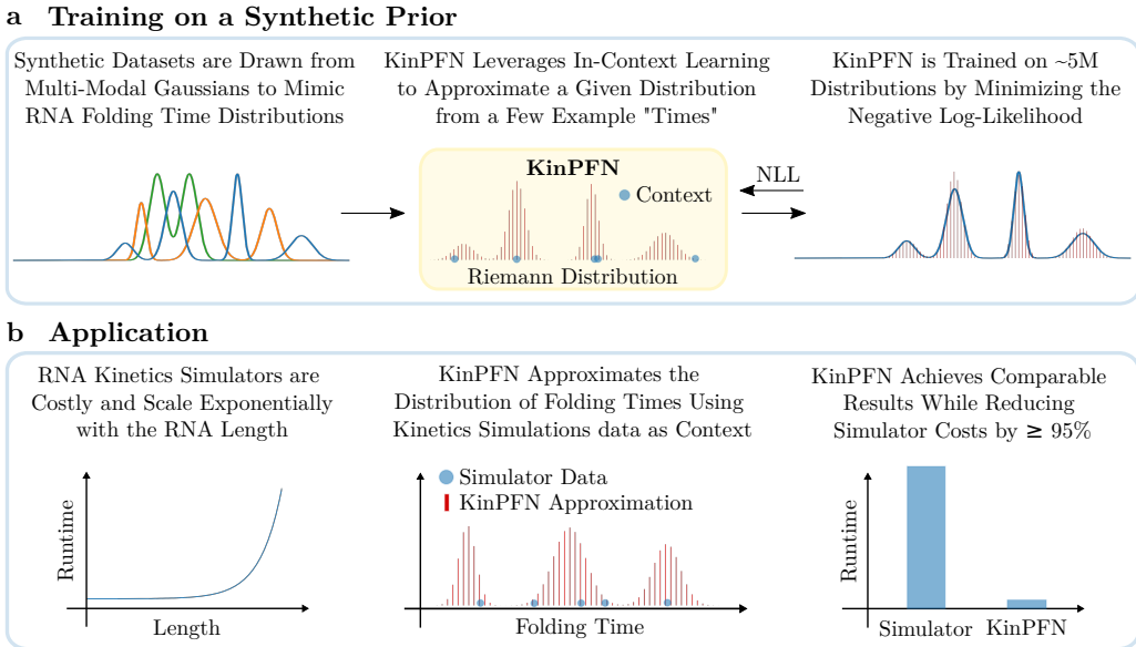
Figure 1: Graphical abstract. a: KinPFN is trained on synthetic RNA folding time distributions drawn from parameterized multi-modal Gaussians by minimizing the negative log-likelihood (NLL). b: KinPFN accelerates RNA kinetics simulators by predicting the RNA folding time distribution in a single forward pass, given a few folding times as context.
