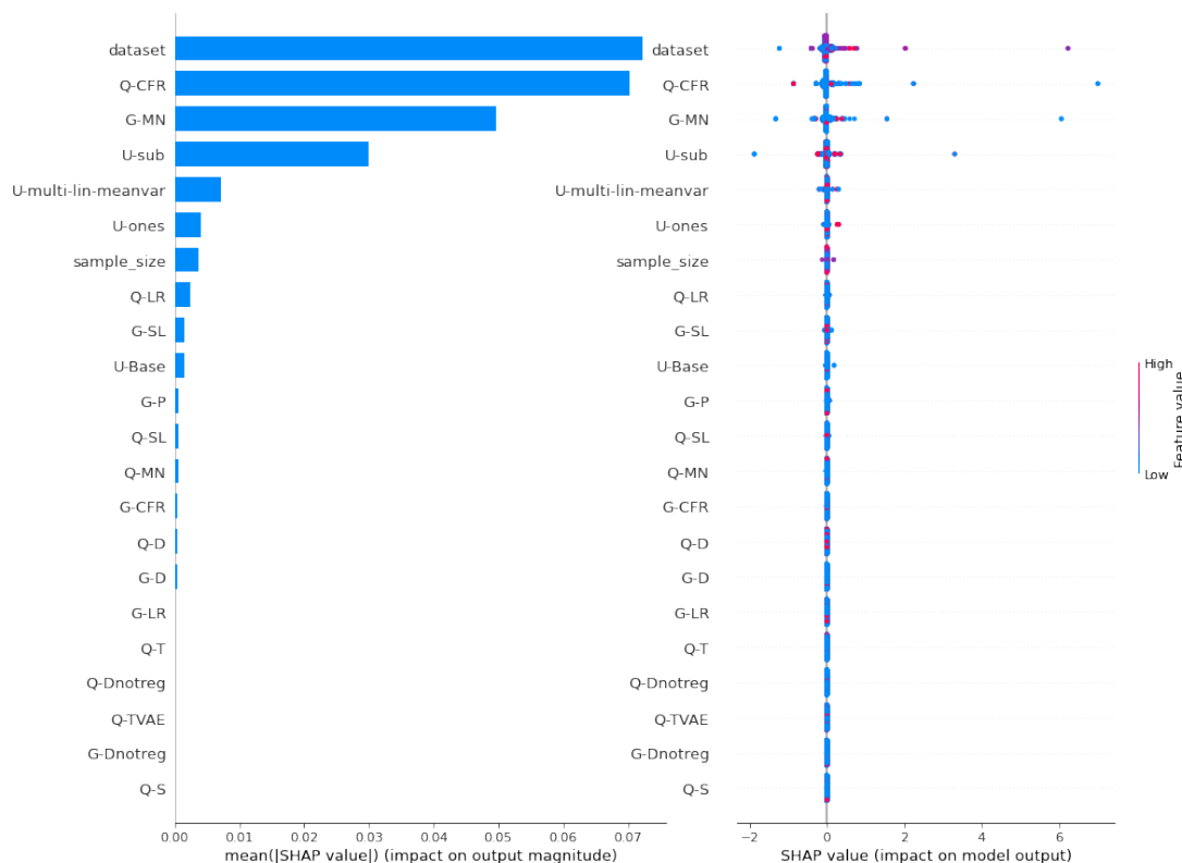
Figure 15: Shapley predictor random forest regressor impact results for the MSE.
