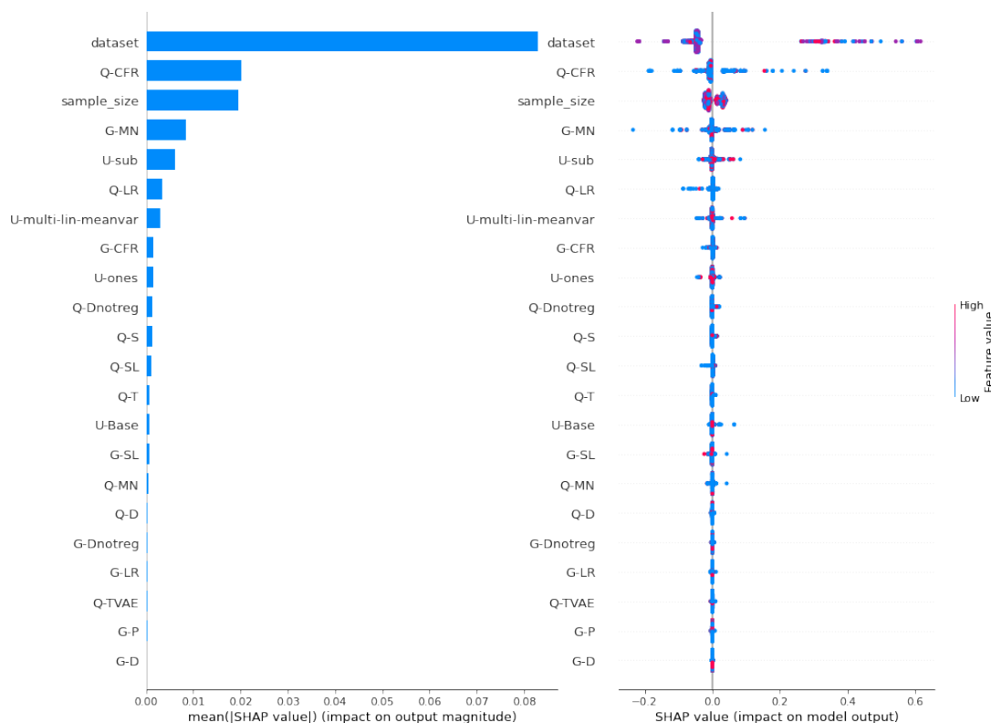
Figure 16: Shapley predictor random forest regressor impact results for the ATE estimate standard error.
