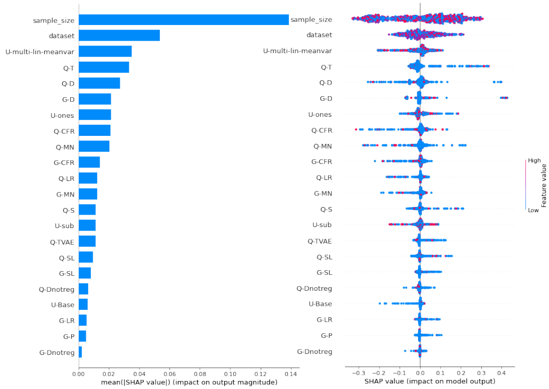
Figure 17: Shapley predictor random forest regressor impact results for the Shapiro-Wilk test p -values.
