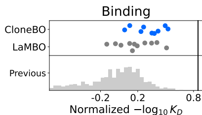
Figure 16: The result of Fig. 6b for affinity with only sequences that were newly measured.
