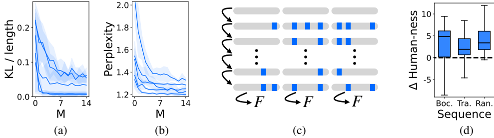
Figure 3: CloneLM is a prior over fitness functions. (a) For 5 different clonal families, with starting sequences X_0 , p_{\text{CloneLM}}(X_{M+1}|X'_{1:M}) gets close to p_{\text{CloneLM}}(X_{M_{\text{large}}+1}|X_{1:M_{\text{large}}}) in KL. We shade one standard deviation across 10 samples of X_{1:M_{\text{large}}} , X'_{1:M} . (b) For 5 different heavy chain clonal families, p_{\text{CloneLM}}(X|X_{0:M}) better predicts sequences in a clonal family when conditioned on more sequences from that same clonal family X_{0:M} . We shade one standard deviation across 10 samples of X_{1:M} . (c) To sample from our prior F | X_0 we perform a martingale posterior procedure. (d) We evolve three antibody therapeutics with three mutations from 25 sampled fitness functions. These sequences evolve to look more like human antibodies.
