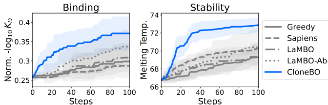
Figure 11: Results of Fig. 5b for various N for representative baselines.
