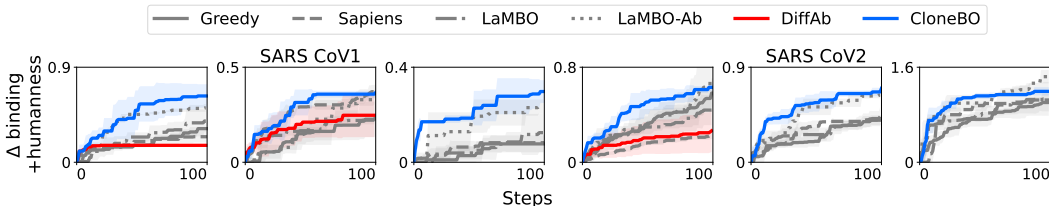
Figure 12: CloneBO efficiently optimizes 6 sequences from CovAbDab for binding to SARS CoV1 (first 3 columns) or CoV2 (last 3 columns). In particular it outperforms a structure-based baseline (DiffAb) for the 3 sequences with an available structure. We show mean and standard deviation achieved across 3 replicates.
