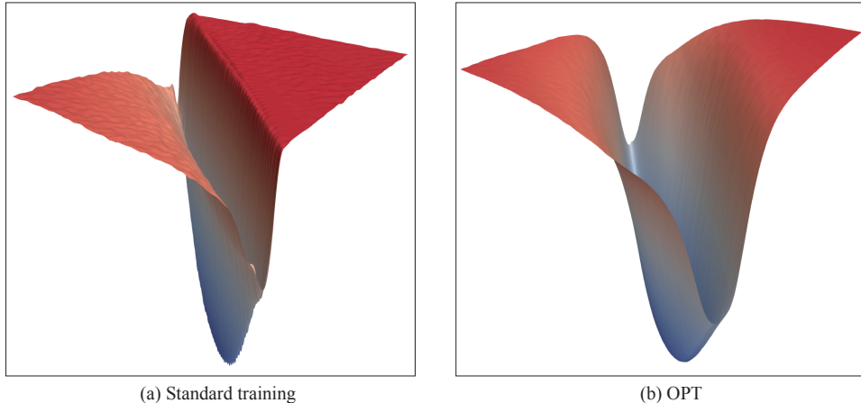
Figure 13: High-quality rendered loss landscapes of standard training and OPT.
