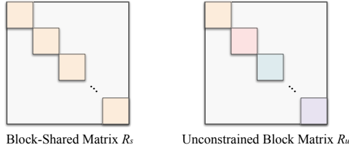
Figure 20: Comparison between the block-shared matrix \mathbf{R}_s and the unconstrained block matrix \mathbf{R}_u .
