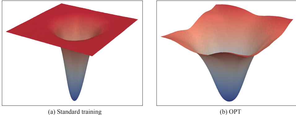
Figure 6: High-quality rendered loss landscapes of standard training and OPT.
