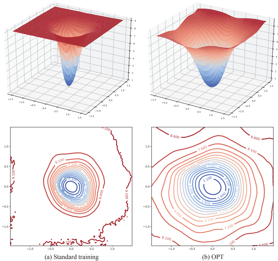
Figure 7: Comparison of loss landscapes between standard training and OPT (full results of Fig. 4(b) in the main paper). Top row: loss landscape visualization with Cartesian coordinate system; Bottom row: loss contour visualization.
