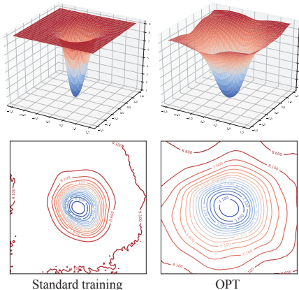
Figure 4: Loss landscape visualization.
