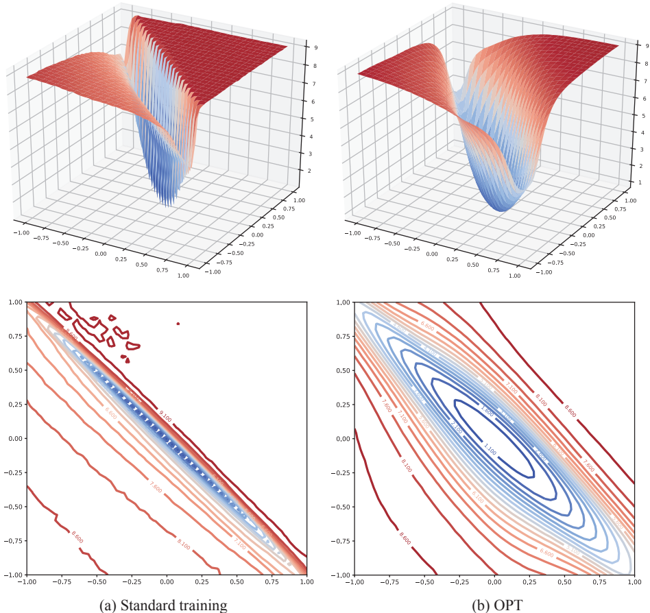
Figure 14: Comparison of loss landscapes between standard training and OPT (full results of Fig. 4(a) in the main paper). Top row: loss landscape visualization with Cartesian coordinate system; Bottom row: loss contour visualization.
