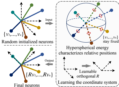
Figure 1: Overview of OPT.
