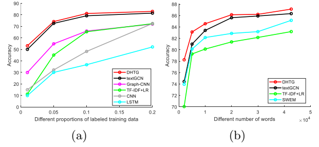
Figure 2: Test accuracy by different (a) sizes of training data and (b) sizes of vocabulary.
