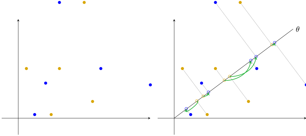
(a) On the left, we can see the two discrete distributions \mu (blue points) and \nu (yellow points). On the right, we have their projections \pi_\theta \# \mu (blue circles) and \pi_\theta \# \nu (yellow circles) along the direction \theta . One then takes the increasing ordering of \pi_\theta \# \mu and \pi_\theta \# \nu , to obtain the corresponding matchings (green arrows) and computes the cost following Eq. 3.
