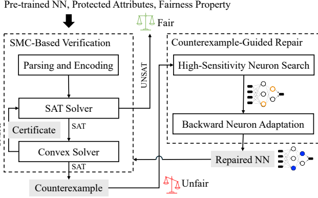
Figure 1: High-level view of the FaVeR workflow.
