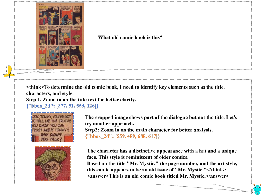
Figure 9: This figure presents how VLM-R 3 performs complex interleaved text-image CoT reasoning.
