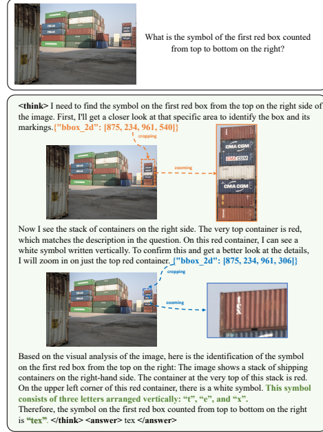
Figure 1: This figure visualizes our proposed VLM-R 3 approach, which integrates region grounding and refinement in an interleaved visual-textual reasoning chain. While conventional text-based reasoning fails when analyzing scenes that require dynamic, iterative, and fine-grained interaction with specific visual regions, our approach succeeds by precisely identifying and focusing on critical visual elements, such as 'the first red box counted from top to bottom on the right' in this example, to derive accurate conclusions through targeted visual reasoning.
