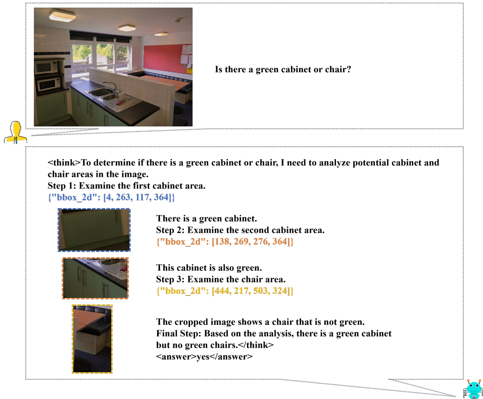
Figure 8: This figure presents how VLM-R 3 iteratively tracks multiple visual cues in an image.
