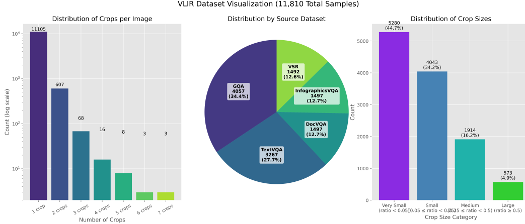
Figure 3: Distribution of the VLIR dataset: (a) number of crops per image, (b) samples across different source datasets, and (c) categorization of crops based on relative size.
