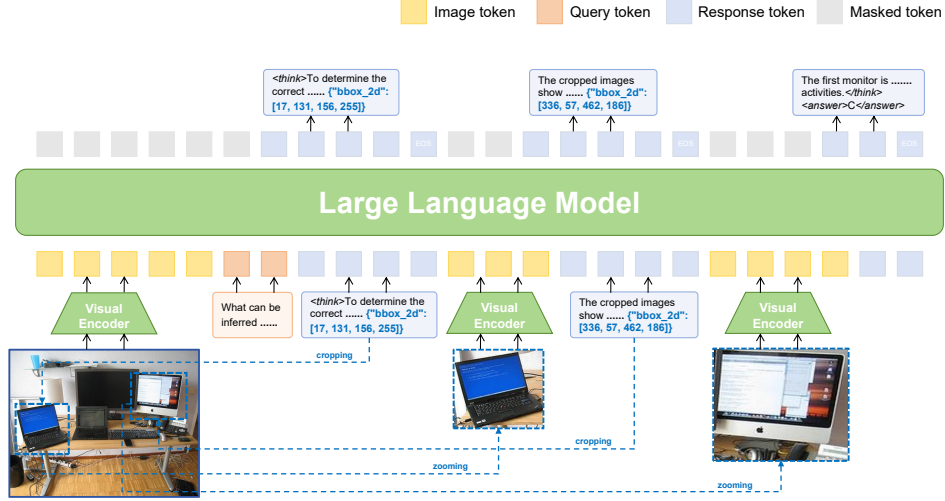
Figure 2: The visualization of the inference pipeline of our proposed methods.
