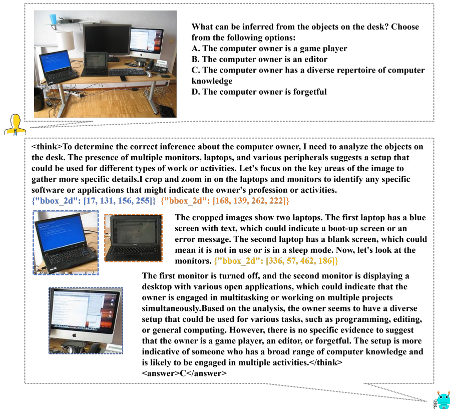
Figure 10: This figure presents how VLM-R 3 performs complex interleaved text-image CoT reasoning.
