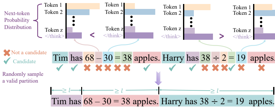
Figure 1: Adaptive stepwise partitioning: step boundaries are identified where the probability of concluding the reasoning chain after the current token, p(\langle /think \rangle | G_i) , is greater than concluding after the subsequent token, p(\langle /think \rangle | G_{i+1}) . A final partition is chosen to meet constraints on step count m and minimum length l .
