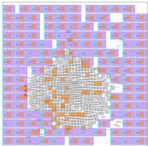
Figure 4: The three domains included in A2Perf: computer chip floorplanning for optimizing integrated circuit layouts, web navigation for automated form filling and website interaction, and quadruped locomotion for robotic control. These specific domains were selected based on their demonstrated transfer from simulation to real-world applications.
