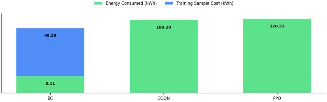
Figure 1: Comparison of energy consumption and training-sample cost for BC, DDQN, and PPO on the Ariane Netlist task, enabled by A2Perf. Note: The plot is not to scale for visibility of smaller values. Online methods (DDQN and PPO) have no training-sample cost because they are initialized without pre-collected data. BC’s energy consumption (0.11 kWh) is significantly smaller than its training-sample cost (48.28 kWh), which represents the energy used to generate the training data.
