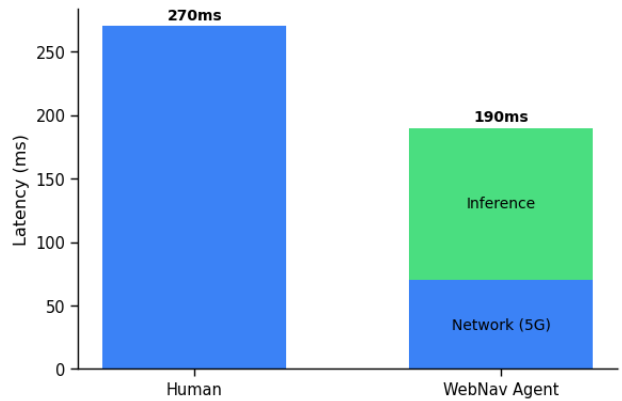
Figure 2: Latency of web-navigation agents compared with typical human reaction time. Even when served from the cloud, the agents respond quickly enough for real-time form-filling and similar interactive tasks.
