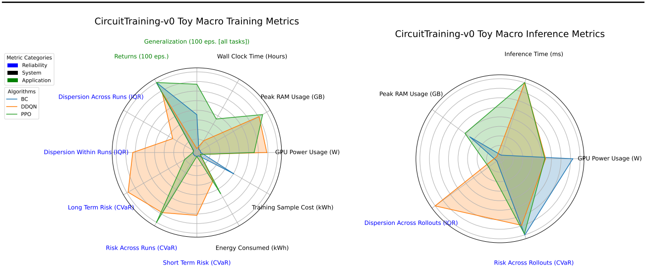
Figure 8: Graphical representation of metrics for the "Toy Macro" netlist task of CircuitTraining-v0
