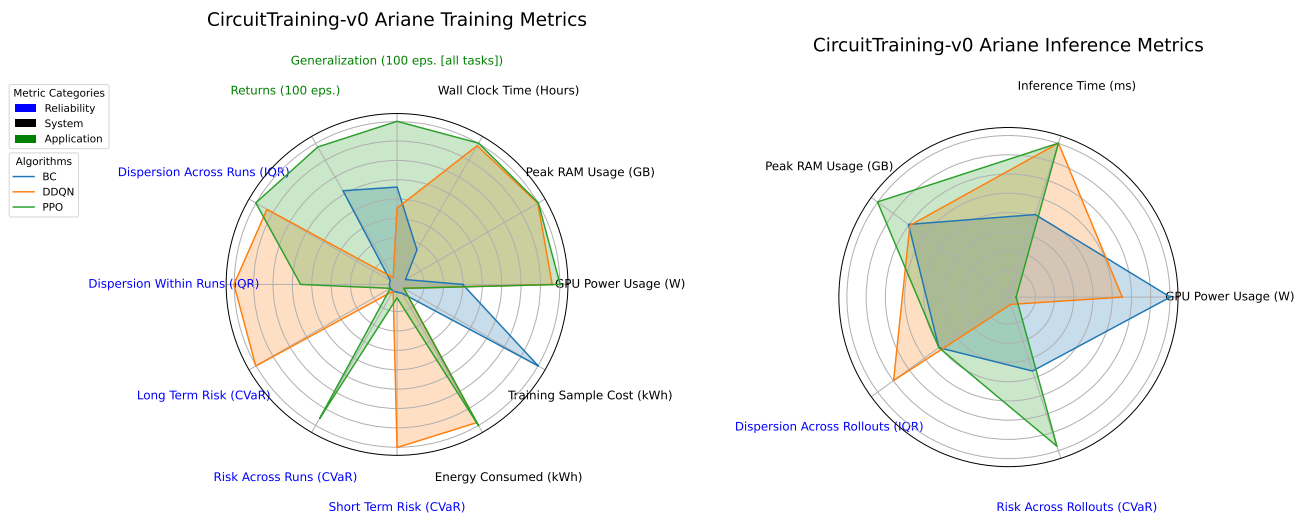
Figure 9: Graphical representation of metrics for the "Ariane" netlist task of CircuitTraining-v0
