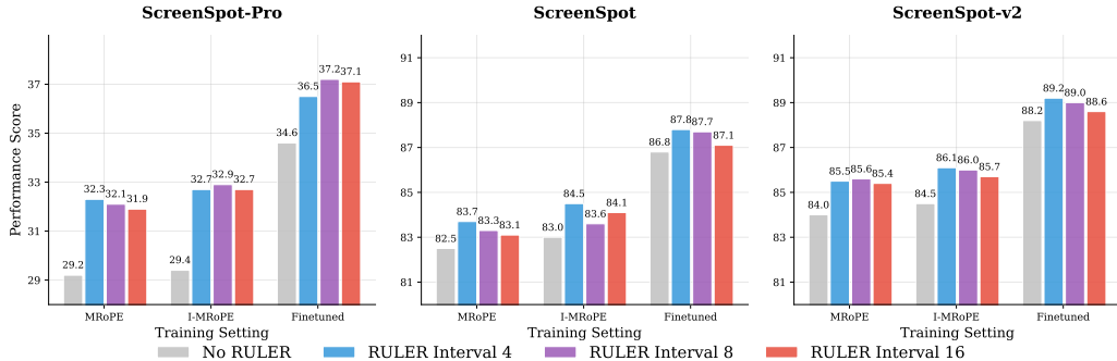
Figure 3: Ablation study on RULER token intervals s across different benchmarks and training settings.
