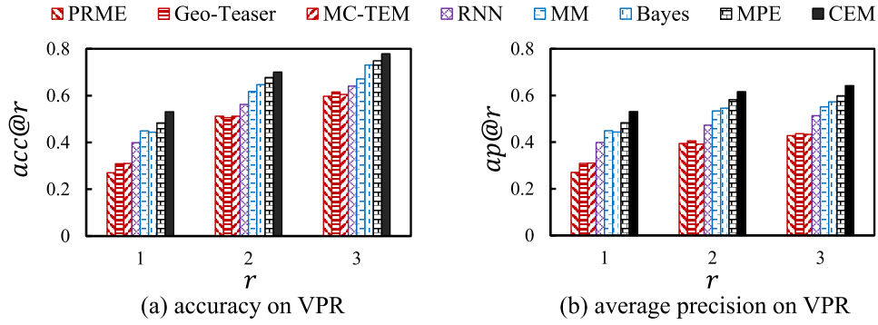
Fig. 4. Performance comparison for next location prediction on VPR data.
