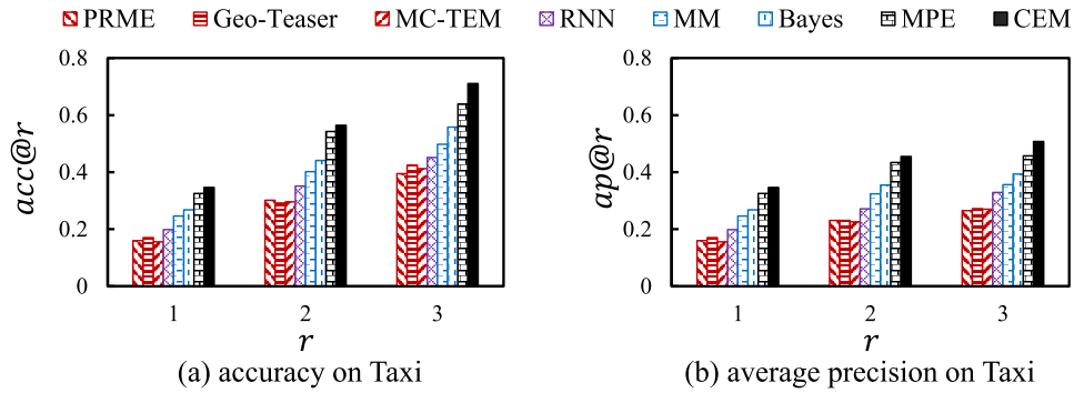
Fig. 5. Performance comparison for next location prediction on Taxi data.
