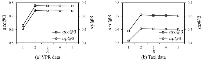
Fig. 6. Effects of varying the number of contextual locations K .
