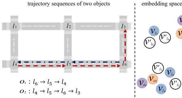
Fig. 2. An illustration of our method CEM. We respectively represent objects o_1 and o_2 with the embedding vectors v_{o_1} and v_{o_2} (denoted by circles with orange background), locations l_4 , l_5 and l_6 taking the role of “contextual locations” with the embedding vectors v_{l_4} , v_{l_5} and v_{l_6} (denoted by circles with blue background), locations l_3 , l_4 , l_5 and l_6 taking the role of “target locations” with the embedding vectors v'_{l_3} , v'_{l_4} , v'_{l_5} and v'_{l_6} (denoted by circles with white background). We use the hour index in a day to represent the time. The time duration between 8 a.m. and 9 a.m. is represented by t_8 , corresponding to the embedding vector v_{t_8} (denoted by the circle with purple background), and the same with the duration between 9 a.m. and 10 a.m. Note that the distance in the embedding space is expected to capture the relatedness among locations, objects or time slots.
