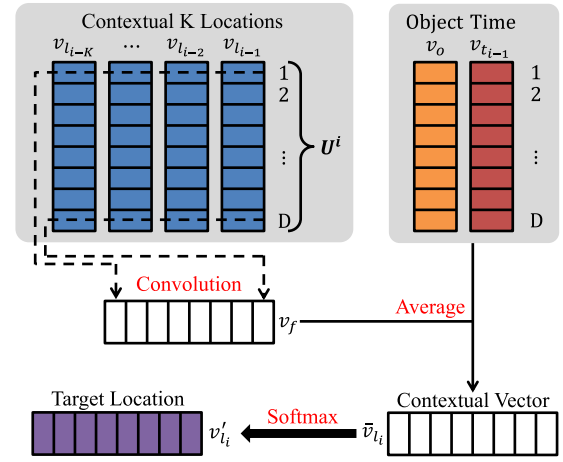
Fig. 3. The architecture of CEM. Orange, blue, purple and red boxes denote the embedding vectors for objects, contextual locations, target locations and time slots, respectively.
