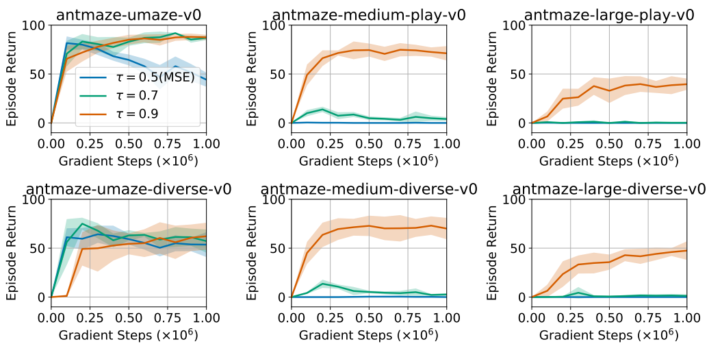
Figure 5: Results on Ant Maze for different values of \tau . Note that \tau = 0.5 corresponds to using the mean squared error instead of expectile regression.
