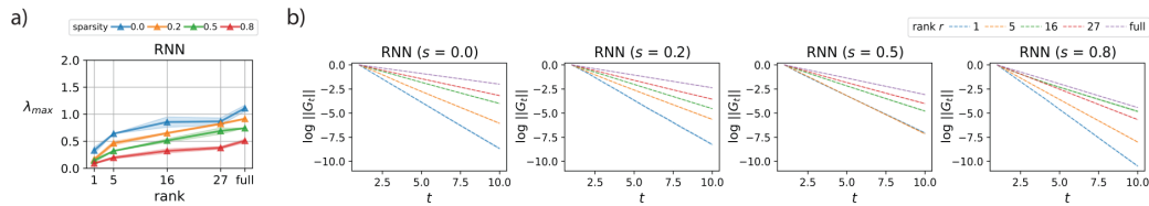
Figure 19: a) Spectral radius of recurrent weights \mathbf{W}_{rec}(r, s) in trained RNN networks across ranks and sparsities. b) Frobenius norm of recurrent gradients \mathbf{G}_t as a function of time. Note that the norms are plotted in log space and translated to decay from 0 to enable easier comparison. For details on the computation, refer to A.11.
