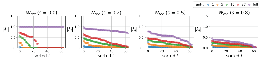
Figure 15: Eigenspectra of orthogonally initialized recurrent weights across various ranks and sparsities sorted in decreasing order.
