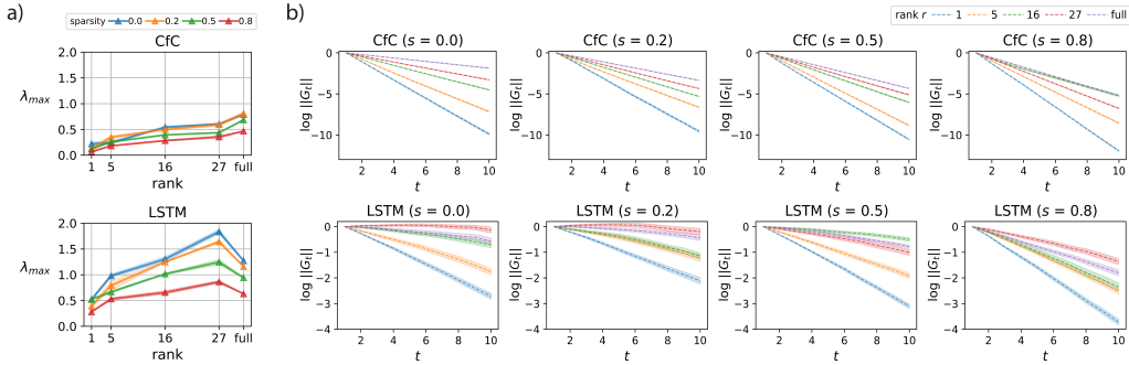
Figure 4: a) Spectral radius of recurrent weights \mathbf{W}_{rec}(r, s) in trained Cfc and LSTM networks across ranks and sparsities ( \pm 1 SE). b) Frobenius norm of recurrent gradients \mathbf{G}_t as a function of time ( \pm 1 SE). Note that the norms are plotted in log space and translated to decay from 0 to enable easier comparison. For details on the computation, refer to A.11.
