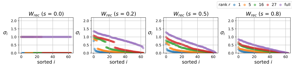
Figure 14: Singular value spectra of orthogonally initialized recurrent weights across various ranks and sparsities sorted in decreasing order.
