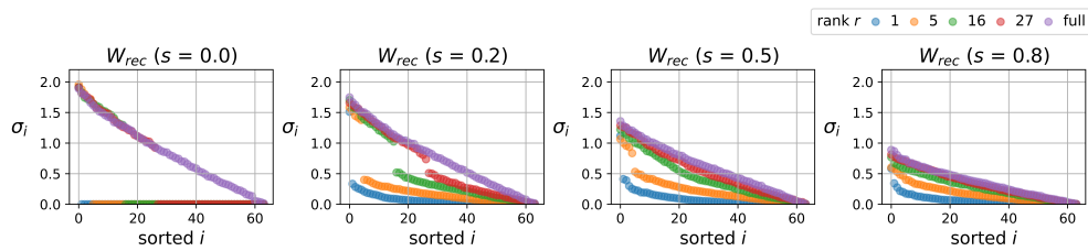
Figure 16: Singular value spectra of Glorot uniform initialized recurrent weights across various ranks and sparsities sorted in decreasing order.
