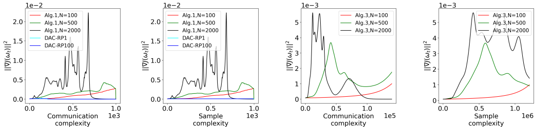
Figure 8: Comparison of optimality gap J(\omega^*) - J(\omega_t) among decentralized AC-type algorithms on cliff navigation.
