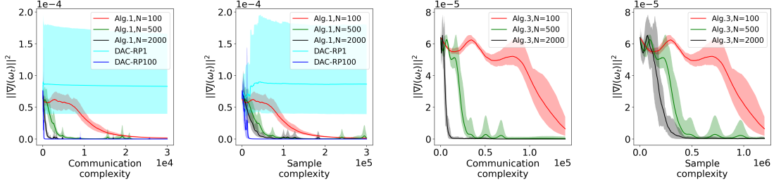
Figure 2: Comparison of \|\nabla J(\omega_t)\|^2 among decentralized AC-type algorithms for ring network .
