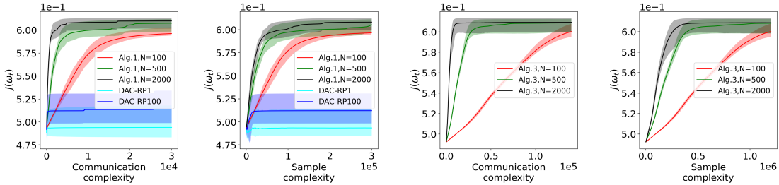
Figure 1: Comparison of accumulated discounted reward J(\omega_t) among decentralized AC-type algorithms in a ring network with sparse connections .
