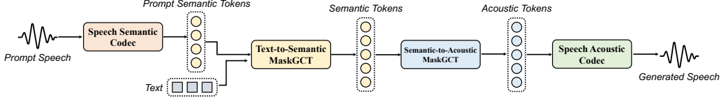
Figure 1: An overview of the proposed two-stage MaskGCT framework. It consists of four main components: (1) a speech semantic representation codec converts speech to semantic tokens; (2) a text-to-semantic model predicts semantic tokens with text and prompt semantic tokens; (3) a semantic-to-acoustic model predicts acoustic tokens conditioned on semantic tokens; (4) a speech acoustic codec reconstructs waveform from acoustic tokens.
