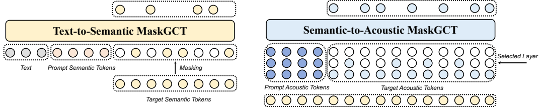
Figure 2: An overview of training diagram of the T2S (left) and S2A (right) models. The T2S model is trained to predict masked semantic tokens with text and prompt semantic tokens as the prefix. The S2A model is trained to predict masked acoustic tokens of a random layer conditioned on prompt acoustic tokens, semantic tokens, and acoustic tokens of the previous layers.
