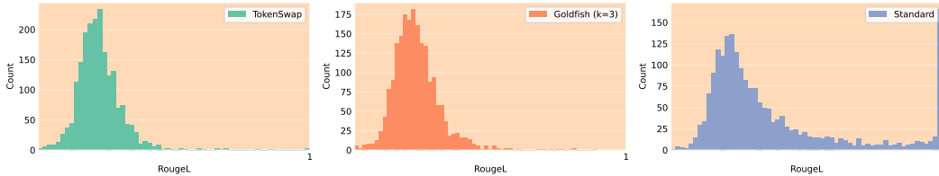
Figure 5: We compare TOKENSWAP with Goldfish [32] on RougeL score distributions for Wikipedia generations. The similar distributions of TOKENSWAP and Goldfish ( k=3 ) demonstrate that our inference-time approach is comparable to expensive pre-training methods in reducing memorization.
