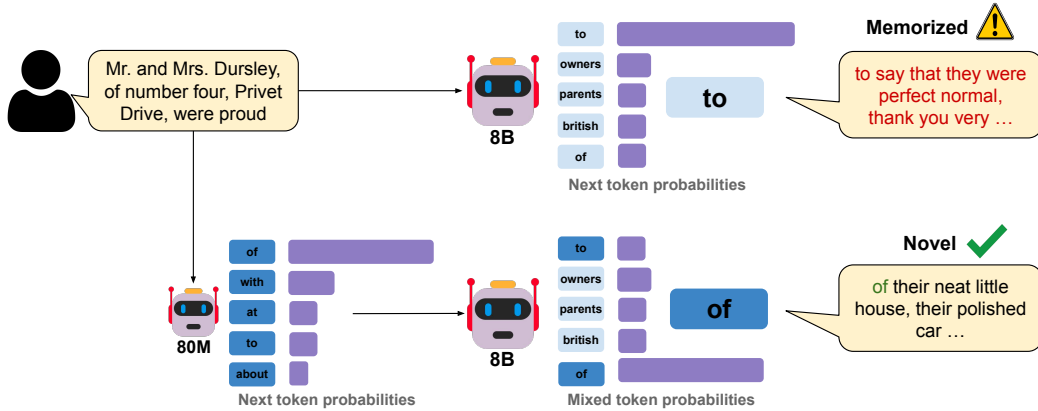
Figure 2: Overview of TOKENSWAP. Our approach replaces token probabilities of high-frequency "grammar-based" tokens with those from a small auxiliary language model. This mitigates memorized generation while maintaining fluency and model performance. The top path shows standard LLM generation, while the bottom path demonstrates how TOKENSWAP alters token selection to disrupt memorization and produce novel text.
