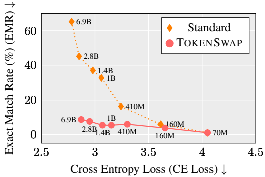
Figure 3: Memorization (EMR) vs Performance (CE Loss) across different model sizes. Larger, more capable models exhibit higher memorization. TOKENSWAP, with Pythia-70M as the auxiliary model, achieves low memorization rates while maintaining competitive performance. Details in Section 3.2
