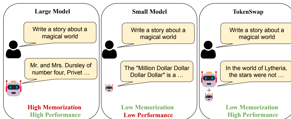
Figure 1: TOKENSWAP combines the strengths of large and small language models. Large models achieve high performance but exhibit high memorization. Small models have low memorization but poor performance (generating incoherent text). TOKENSWAP achieves both low memorization and high performance by selectively swapping token probabilities, generating novel, fluent text.
