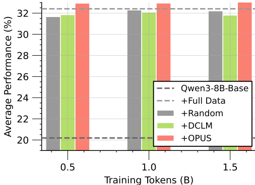
Figure 3: Continued pre-training on SciencePedia. Average performance versus CPT tokens for random CPT, DCLM, and OPUS. Detailed domain-specific results are in Figure 7.
