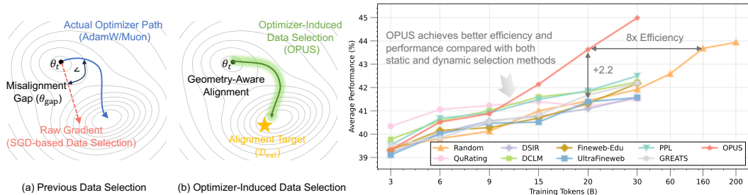
Figure 1: Left: Comparison of different data selection methods. Right: OPUS outperforms random selection by an average of 2.2% accuracy across 10 downstream benchmarks and achieves 8× reduction in computation on GPT-XL using FineWeb dataset.
