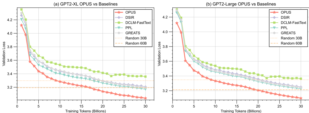
Figure 6: Validation-loss curves on GPT-2 XL and GPT-2 Large pre-trained from scratch on FineWeb-Edu dataset. Left: Results on GPT-2 XL. OPUS compared with representative baselines trained on the high-quality pool, with Random 60B shown as a non compute-matched reference. Curves are shown up to 30B update tokens for compute-matched comparison. Right: Results on GPT2-Large.
