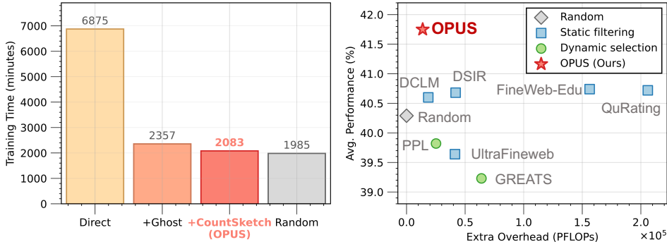
Figure 4: Efficiency and computational cost analysis. Time (minutes) and total compute (PFLOPs) are evaluated on GPT-2 XL after pre-training on FineWeb (30B tokens) with Muon.
