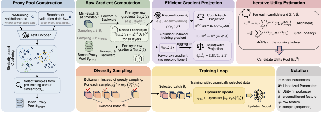
Figure 2: Overview of OPUS pipeline.
