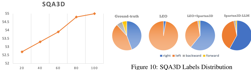
Figure 9: Scaling Effect on SQA3D.
