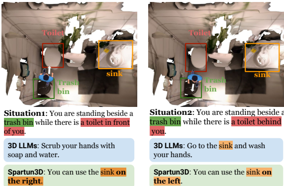
Figure 1: Illustration of situated scene understanding of Spartun3D-LLM compared to other 3D-based LLMs.
