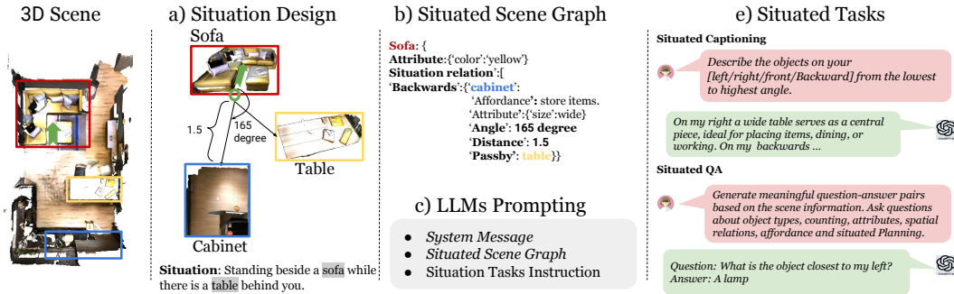
Figure 3: Illustration of Spartun3D Dataset Construction Process. Given a 3D scene: a) we first select a pivot object (e.g., sofa) and a referent object (e.g., table) to define the situation; b) we create situated scene graph based on situation, incorporating various spatial relationships (See Fig. 5); c) we use the scene graph to prompt GPT-4o (shown in gray box) to generate data; e) we utilize different prompting strategies for generating situated captions and QA pairs.
