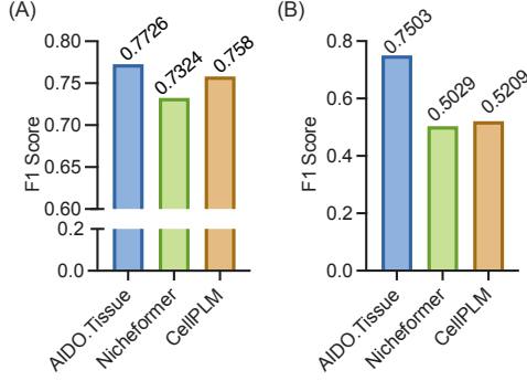
Figure 3. Cell type (A) and niche type (B) prediction performance comparison with F1 score metric.
