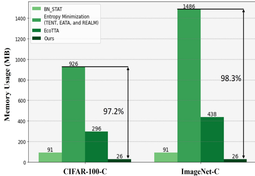
Figure 4: Comparison of memory usage in a single iteration on CIFAR-100-C and ImageNet-C datasets.
