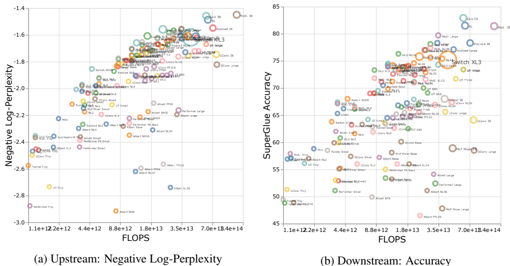
Figure 1: An overview compute-performance (FLOPs vs performance) plot of all the diverse models and architectures we pretrained and finetuned in this study. Colors represent different model architectures and size of the circles represent the size of the model (parameters).
