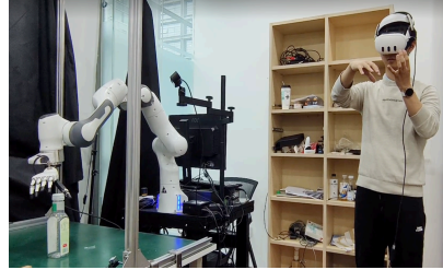
Figure 6: Overview of the teleoperation system setup.
