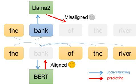
Figure 1: Key Differences between BERT and Llama2 Language Models. Blue and red lines indicate the information flows of understanding and predicting.
