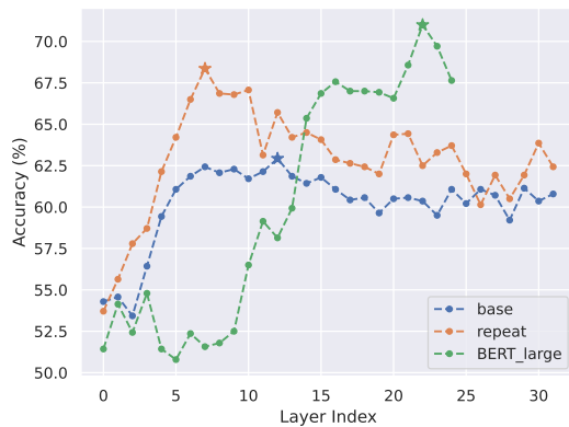
Figure 2: Layer-wise accuracy for different settings and models. Star shows the best value.
