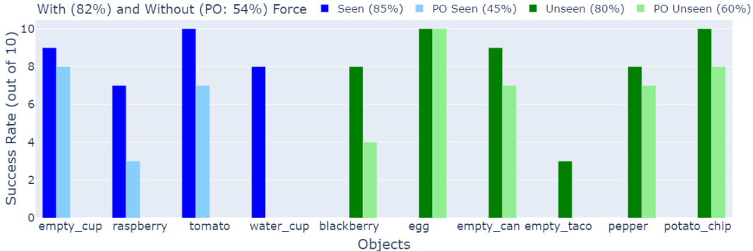
Figure 2: We conduct a series of 10 trials for a selection of 10 objects; four seen in training, six unseen. Forceful policies (82%) replicate seen grasps (85%) and generalize to similar but unseen objects (80%). position-only policies (54%) retain a level of performance on seen (45%) and improve on unseen (60%) delicate objects, suggesting that continuous gripper position control alone contributes to successful delicate grasps. We note that position-only policy failures are generally deforming and compress more than forceful policies (see Fig. 3)
