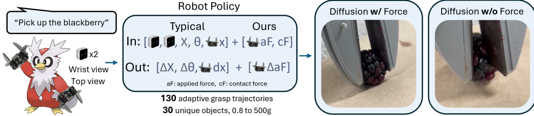
Figure 1: We leverage LLM-directed expert demonstrations [10] of delicate objects to generate a dataset of 130 successful grasps of 30 different objects spanning a variety of physical properties. Our trajectories, unlike other datasets used in end-to-end learning [3, 6], contain observed gripper applied and contact force and the action of increased gripper applied force. We train diffusion policies [9] on the dataset with and without force data and observe that forceful policies can, despite limited data, replicate trained behavior and generalize to unseen delicate objects at 4x reduced latency relative to LLM-policies, and position-only policies cannot.
