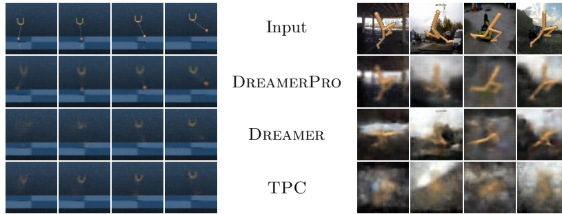
Figure 4: Visualization of learned latent states through reconstruction from an auxiliary decoder. The first row shows the inputs, and the remaining rows show the reconstruction from the RSSM state z_t for each model.
