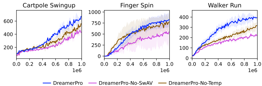
Figure 5: Ablation study. Both \mathcal{J}_{\text{SwAV}}^t and \mathcal{J}_{\text{Temp}}^t are necessary for achieving good performance.
