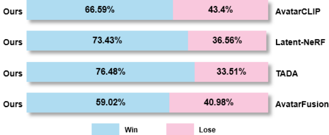
Figure 4: Quantitative results. Our method and methods [8, 21, 19, 10] are evaluated by using the method [15] to measure the visual quality of the generated 3D content, where higher scores are better.
