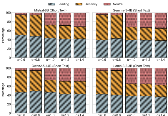
Figure 2: Distribution of positional bias types (Leading, Recency, Neutral) across varying \alpha thresholds for short texts. Each subplot corresponds to a different language model.
