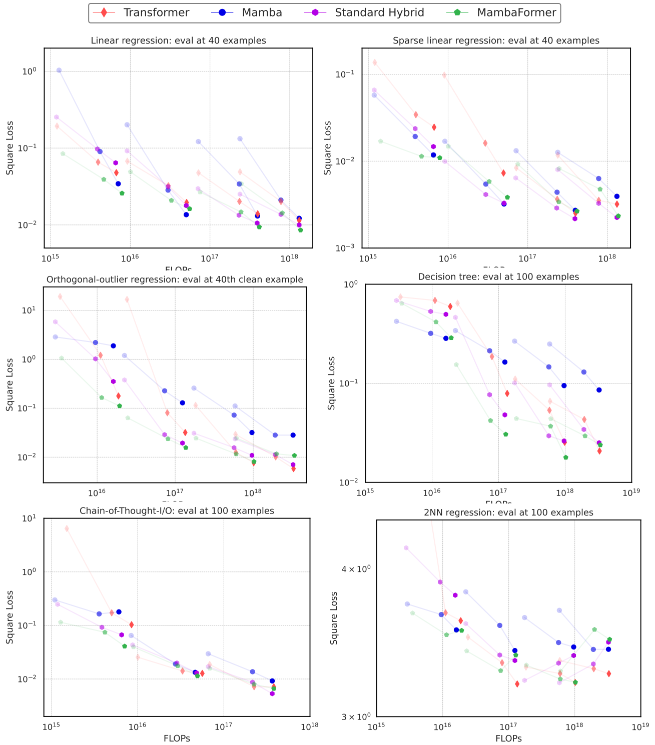
Figure 8. A suite of ICL tasks ran for Transformer, Mamba, and hybrid architectures where each color represents a different architecture. More transparent points indicate earlier stages of training; plotted models are trained {100k, 300k, 500k} iterations. Standard Hybrid and MambaFormer are hybrid models of Transformer and Mamba defined in Section 5.
