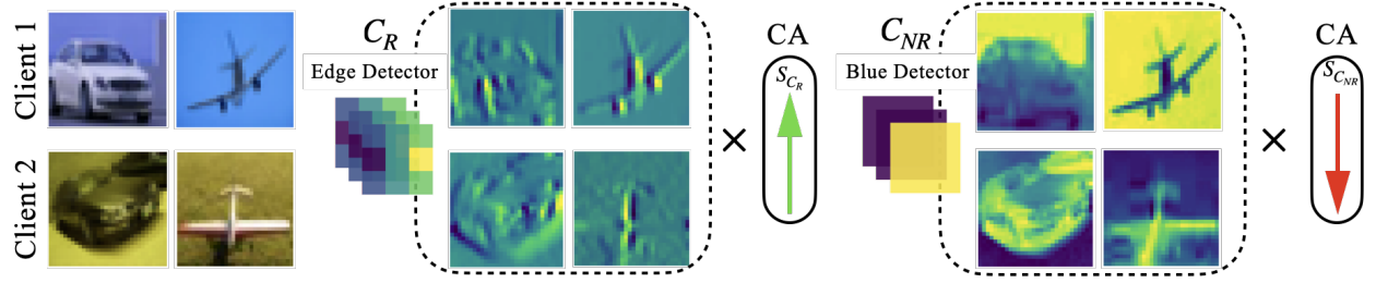
Figure 1: Illustrating how Channel Attention (CA) can boost C_R and suppress C_{NR} . Left: the two clients have heterogeneous datasets. Middle: an edge detector is robust to this feature shift; the activations are consistent for both clients. Right: a blue detector is not robust and its activations cause conflicting gradients.
