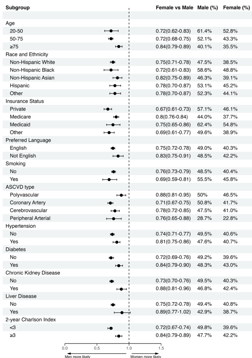
Fig. 5. Subgroup analysis of association between sex and rate of high-intensity statin prescription.
