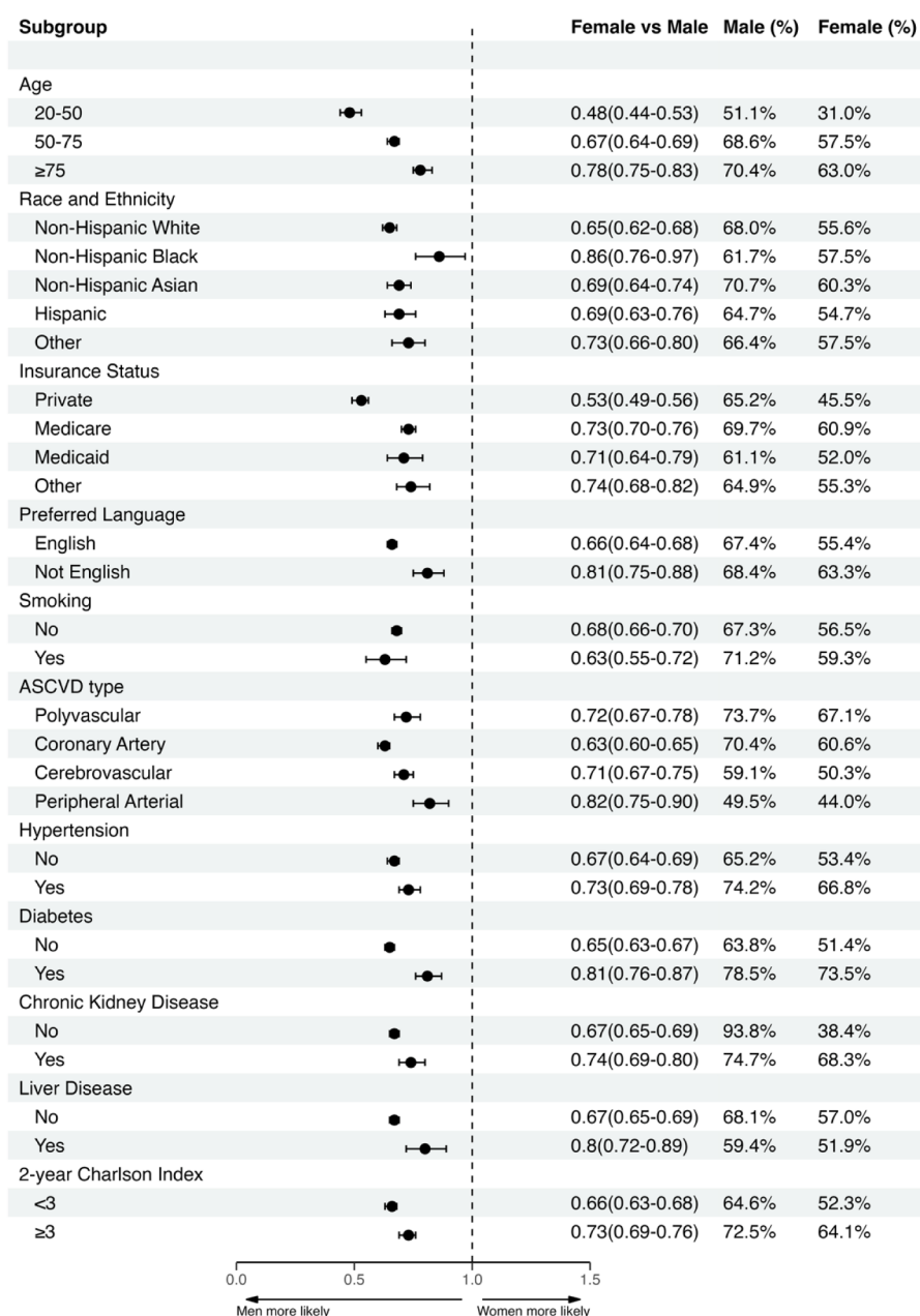
Fig. 4. Subgroup analysis of association between sex and statin prescription.
